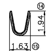
SECTION A-A SCALE 6:1
